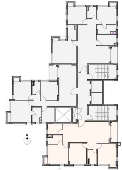
TYPICAL FLOOR PLAN (BLOCK B)
