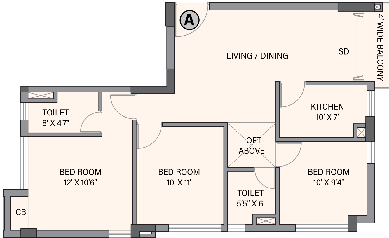
TYPICAL FLOOR PLAN : FLAT- A
