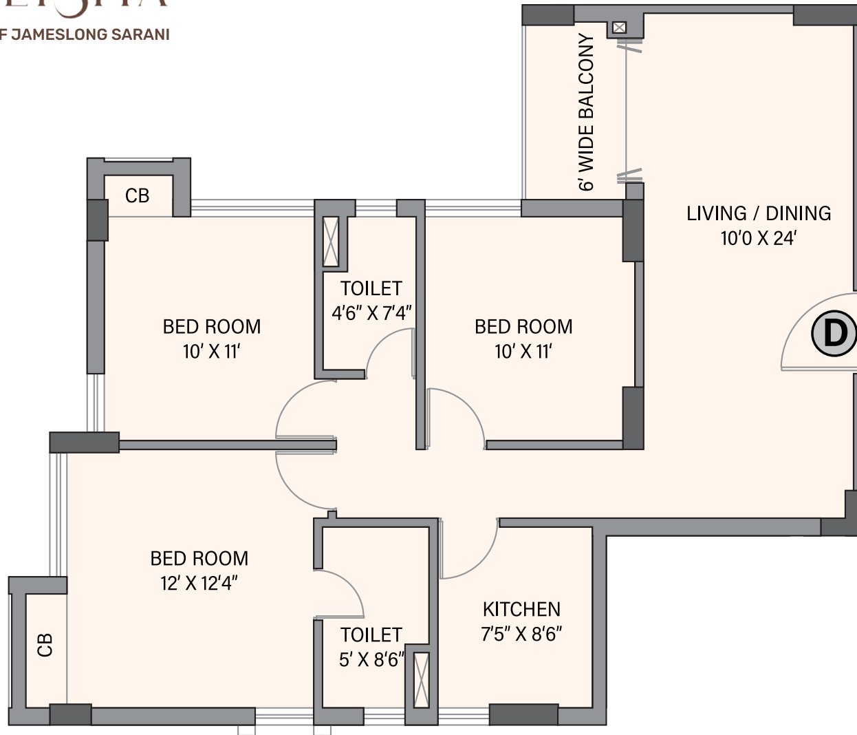
TYPICAL FLOOR PLAN : FLAT- D
